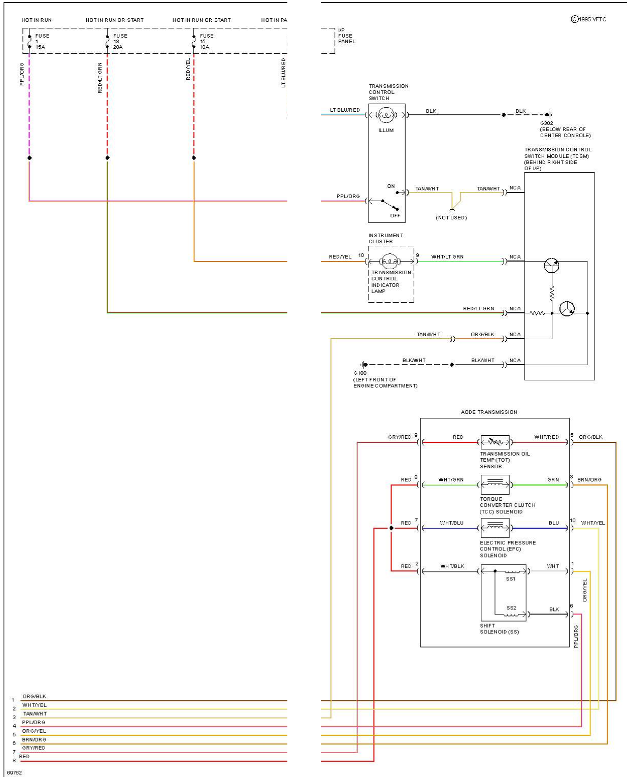
Fig. 4: EEC-IV Wiring Diagram (4 Of 4)
