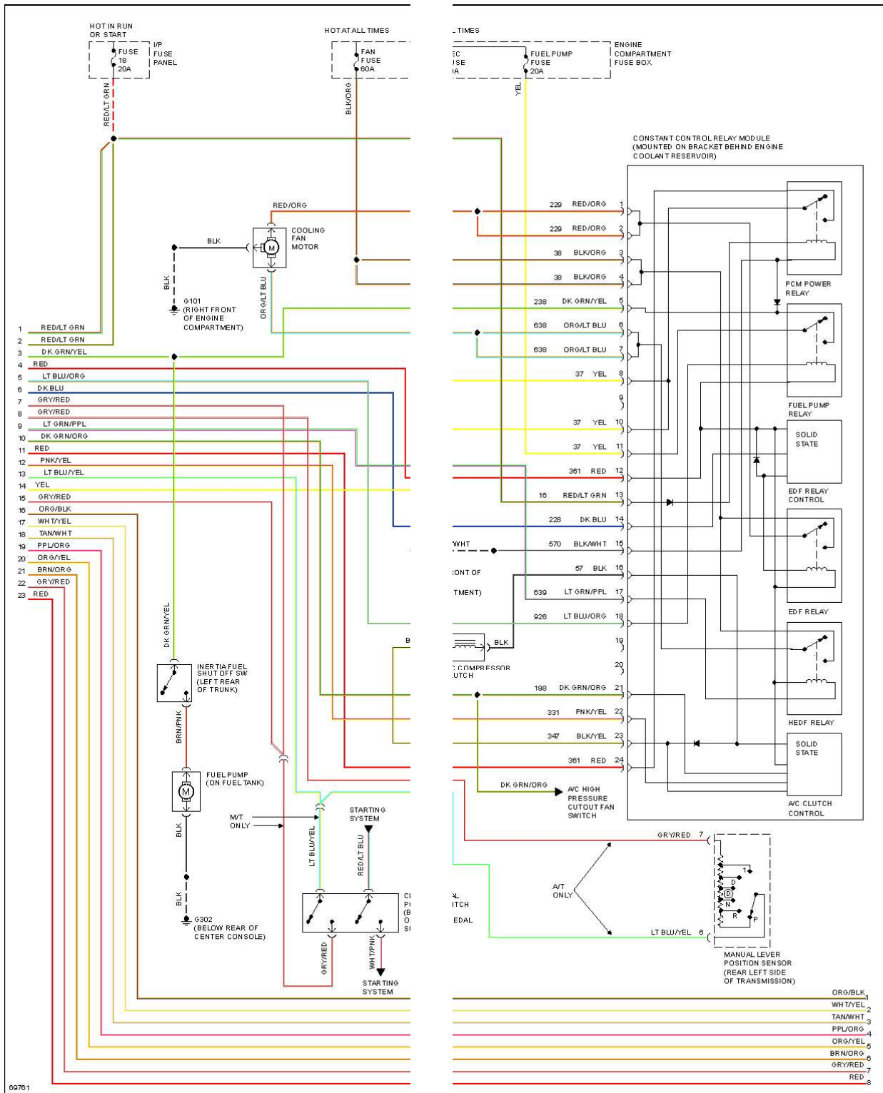
Fig. 3: EEC-IV Wiring Diagram (3 Of 4)
