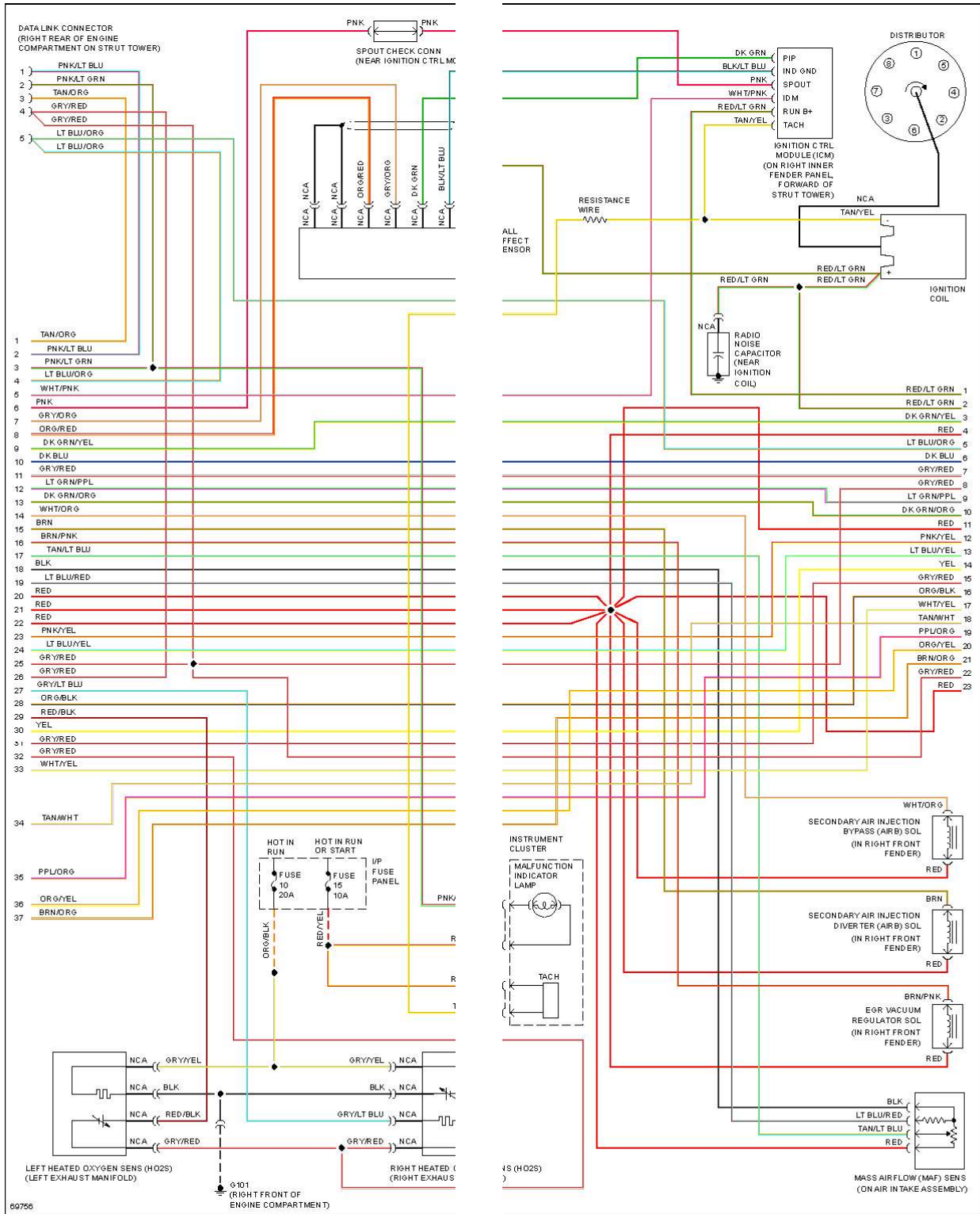
Fig. 2: EEC-IV Wiring Diagram (2 Of 4)
