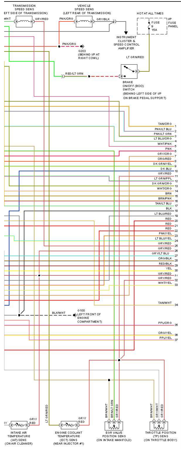
Fig. 1: EEC-IV Wiring Diagram (1 Of 4)
